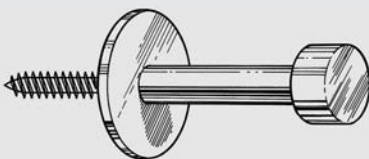
2" DIA BACKPLATE x 2¾" PROJECTION 1" DIA FRONT END
